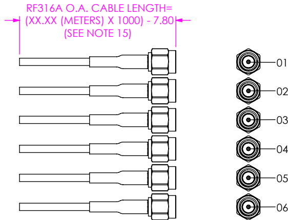
-04: 6 POS (6 X RF316A-01SP1-SING-XXXX)
