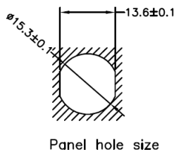
Panel hole size
