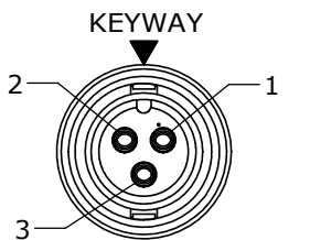
FACE VIEW P/N: CA63803SXXX90
