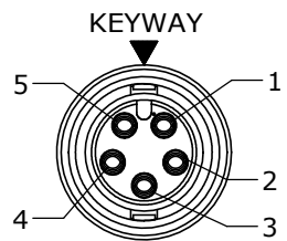
FACE VIEW P/N: CA63805SXXX90
