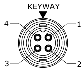
FACE VIEW P/N: CA63804SXXX90
