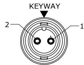
FACE VIEW P/N: CA63802SXXX90
