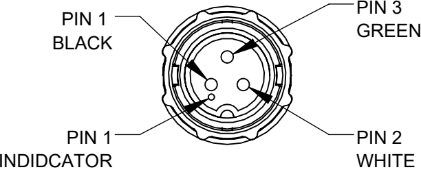
CAEN3C3M1607990 3-PIN MALE
