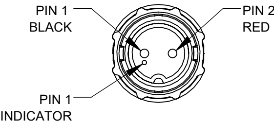
CAEN3C2M1607990 2-PIN MALE
