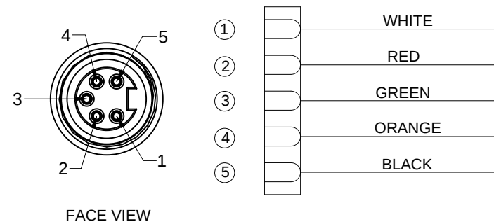
P1 WIRING DIAGRAM
