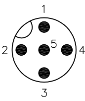
Contact Layout Male
