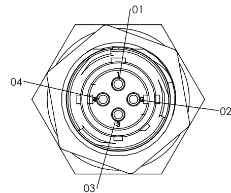
-03: 4 POS (Ø 1.5 TERMINALS)
