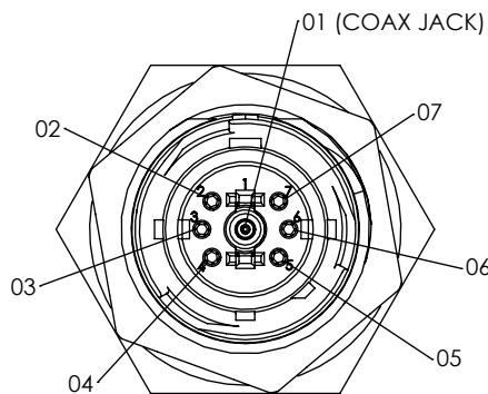
-07: 7 POS COMBO (1 X COAX JACK) (6 X Ø1.0 SOCKETS)
