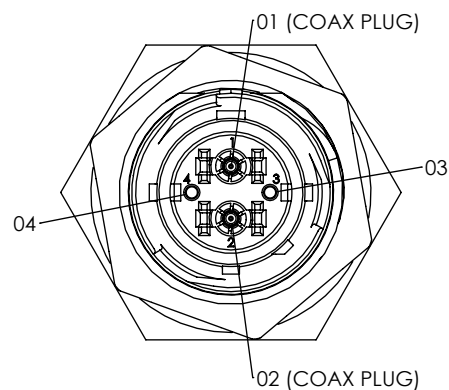
-04: 4 POS COMBO (2 X COAX PLUGS) (2 X Ø 1.0 TERMINALS)
