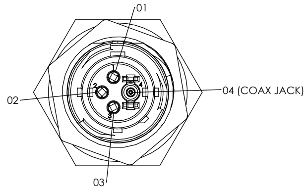
-05: 4 POS COMBO (3 X Ø1.5 SOCKETS) (1 X COAX JACK)
