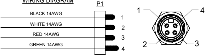
WIRING DIAGRAM
