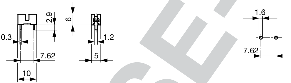
Drilling diagram
