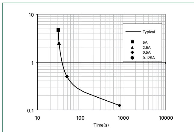
Figure 1. Thermal Characteristics
