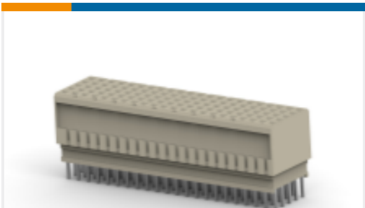
TE Part #5106774-1 Hard Metric Backplane Receptacle Connector: Mezzanine, 2mm
