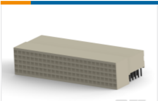
TE Part #352152-1 HM Receptacle Connector: Traditional Backplane, Coplanar, 2mm
