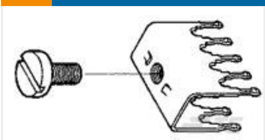
TE Part #5055558-3 10 PWR TAP CONT PLTD STD .100
