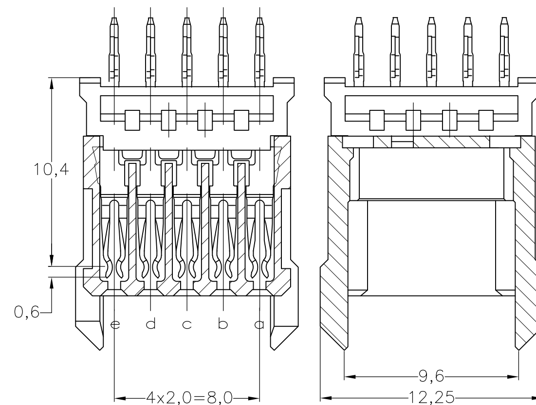
SECTION B-B
