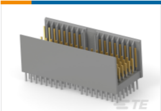
TE Part #5646530-1 Z-PACK 2MM HM TYPE A/B 127P
