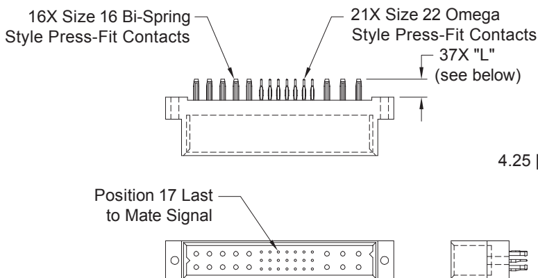
CONNECTOR DIMENSIONS
