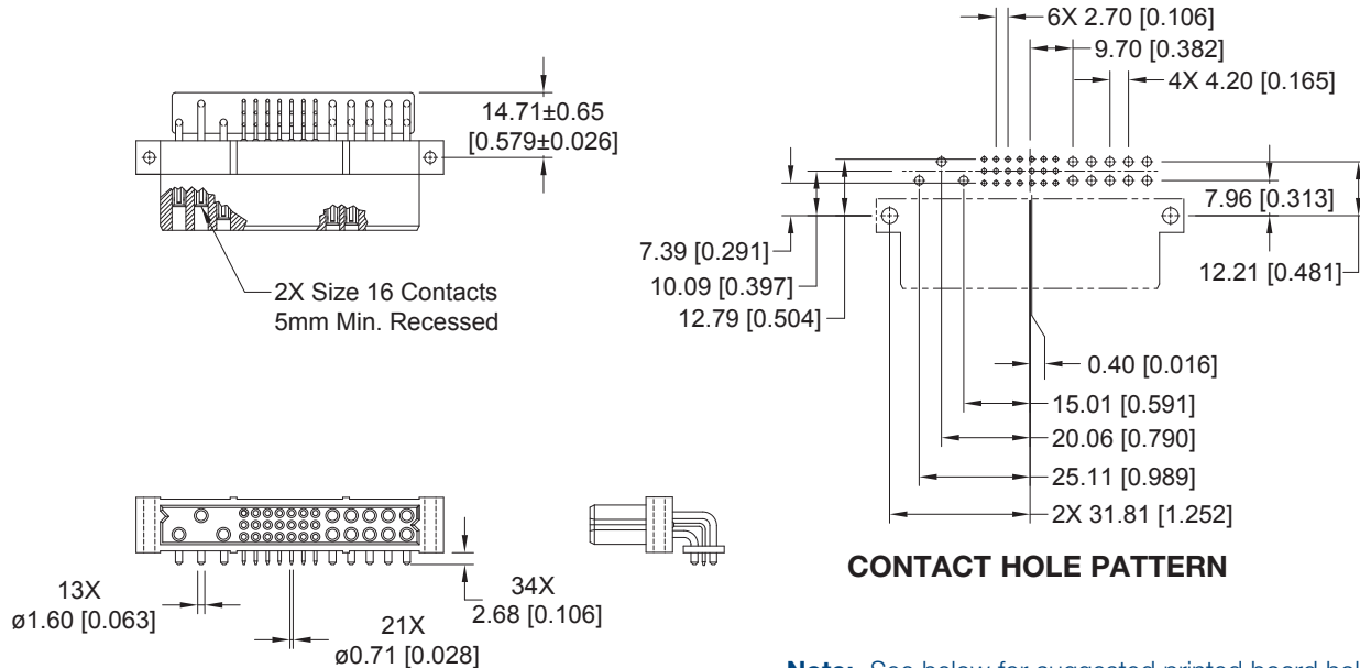
CONNECTOR DIMENSIONS
