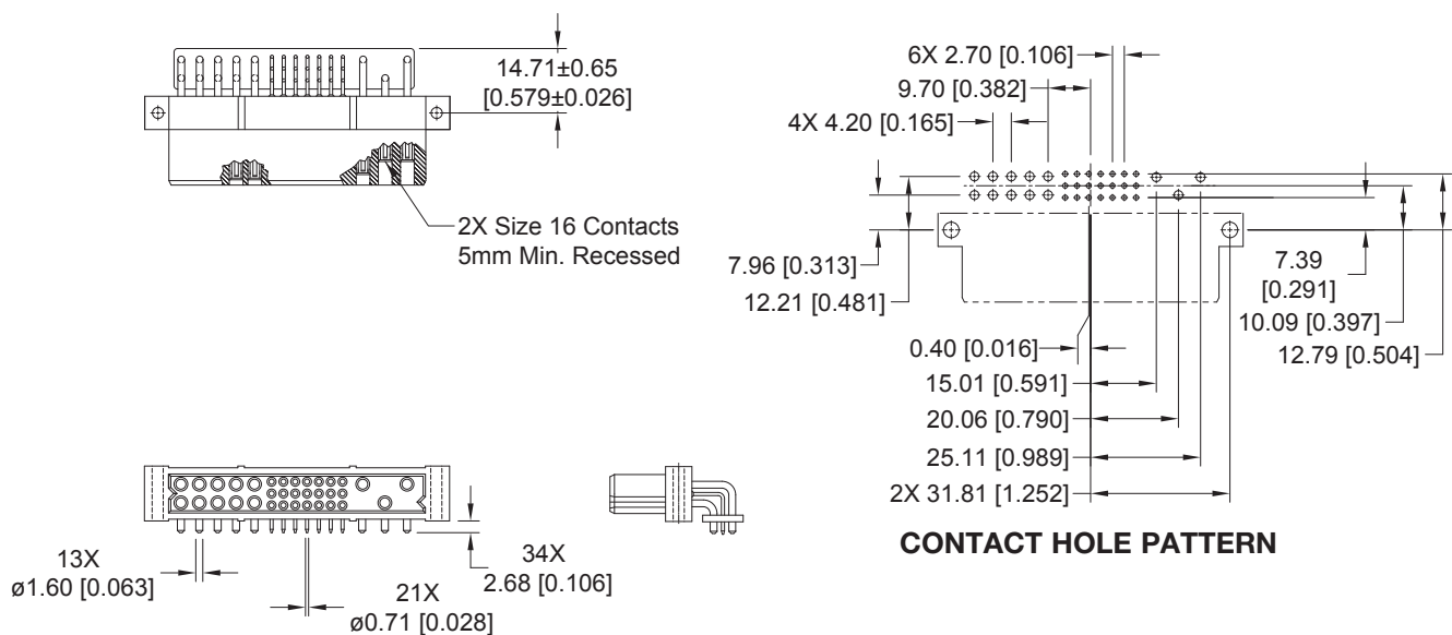
CONNECTOR DIMENSIONS
