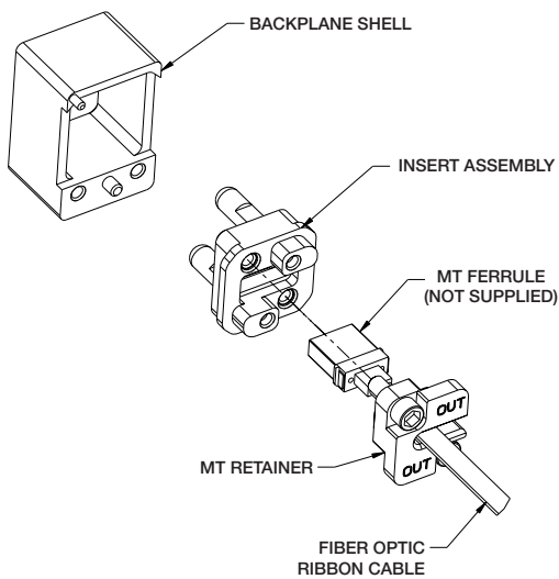
REAR EXPLODED ASSEMBLY VIEW
