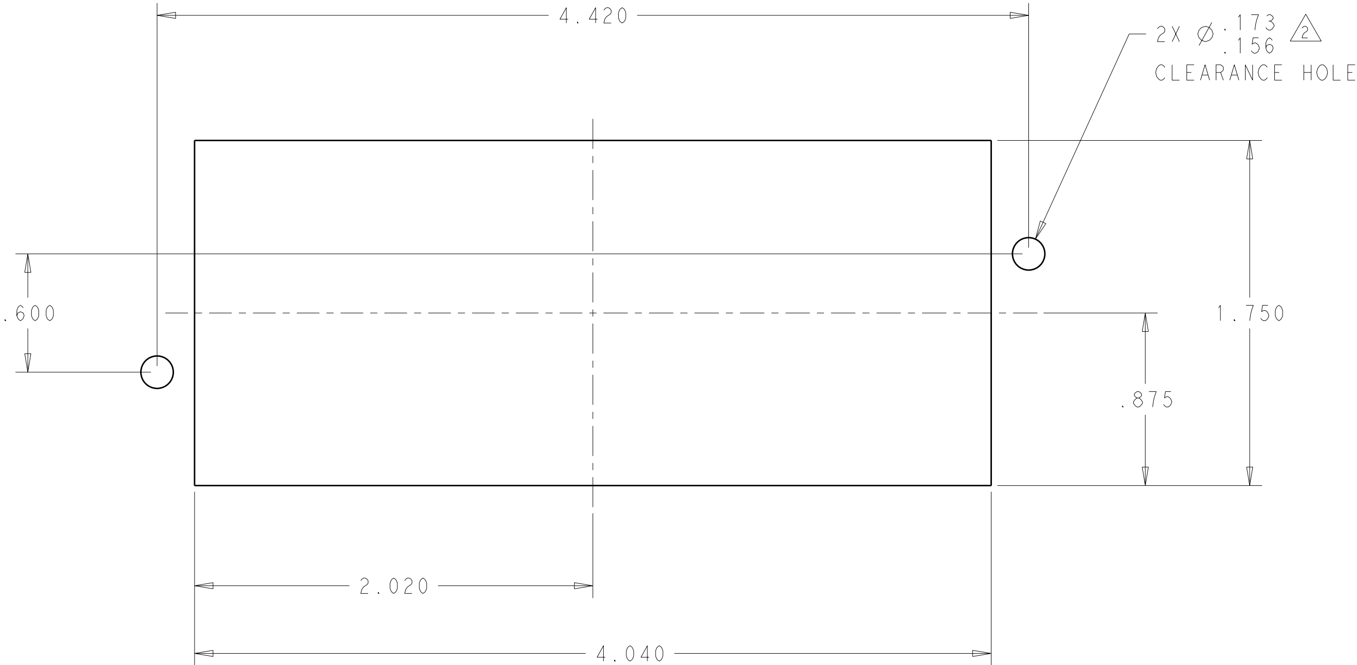
PIN CONNECTOR PANEL CUT-OUT
