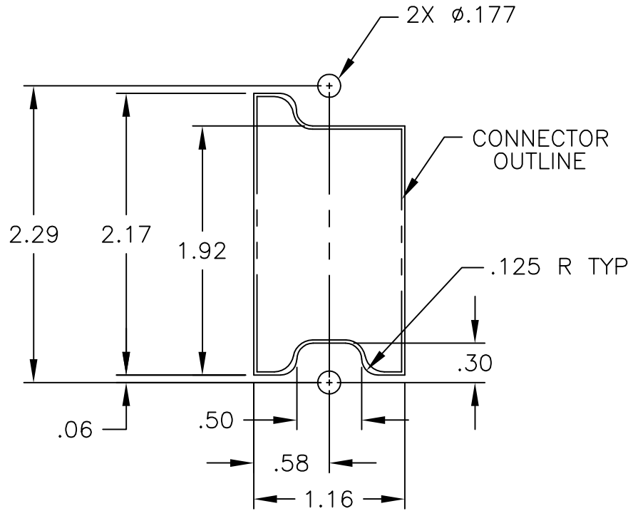
PANEL CUTOUT (VIEWED FROM FRONT OF CONNECTOR)
