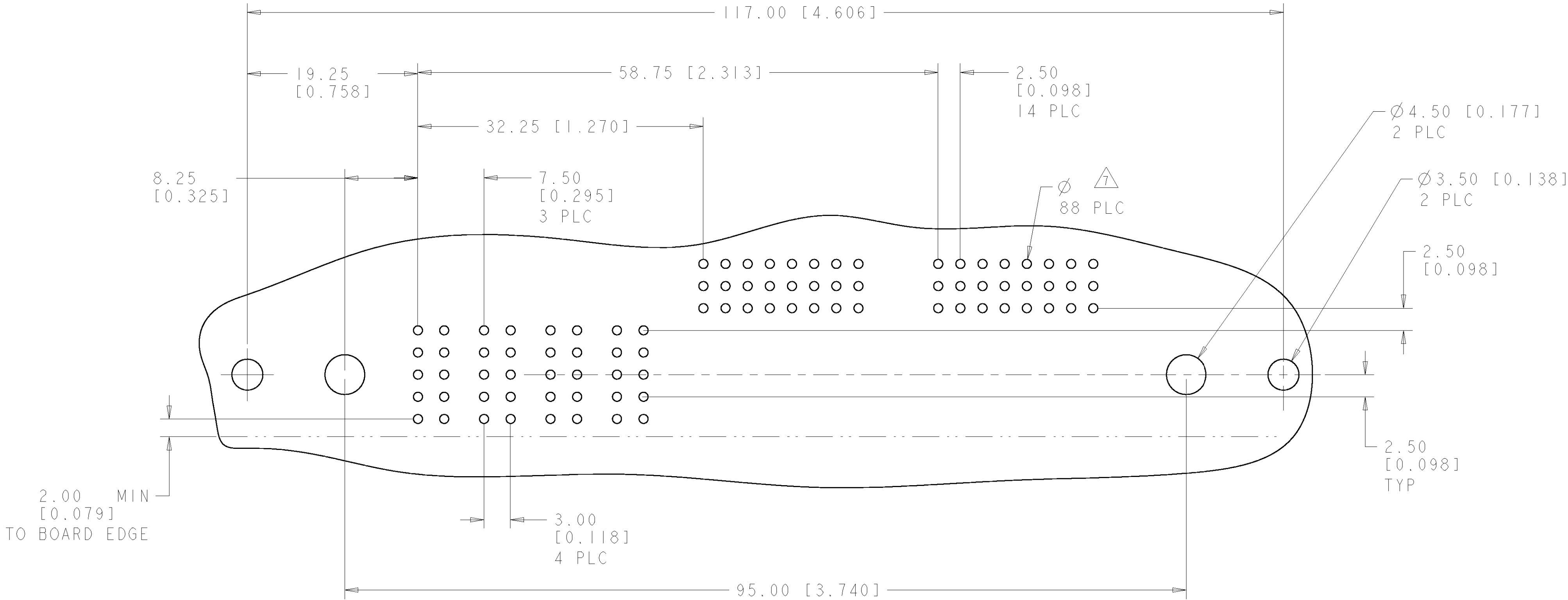
PRINTED CIRCUIT LAYOUT COMPONENT SIDE
