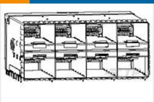
TE Part #1-2180324-9 zSFP+ STACKED 2X4 RECEPTACLE ASSEMBLY
