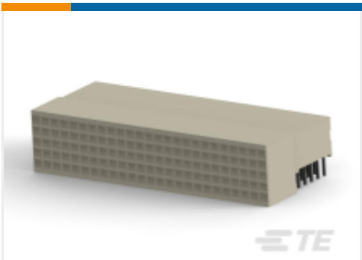
TE Part #5352068-1 HM Receptacle Connector: Traditional Backplane, Coplanar, 2mm
