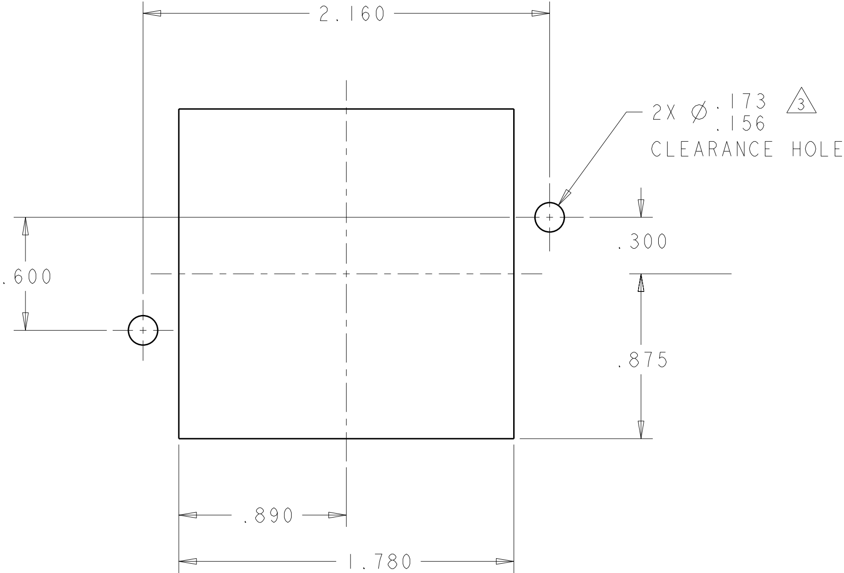
PANEL CUT-OUT COMPONENT SIDE
