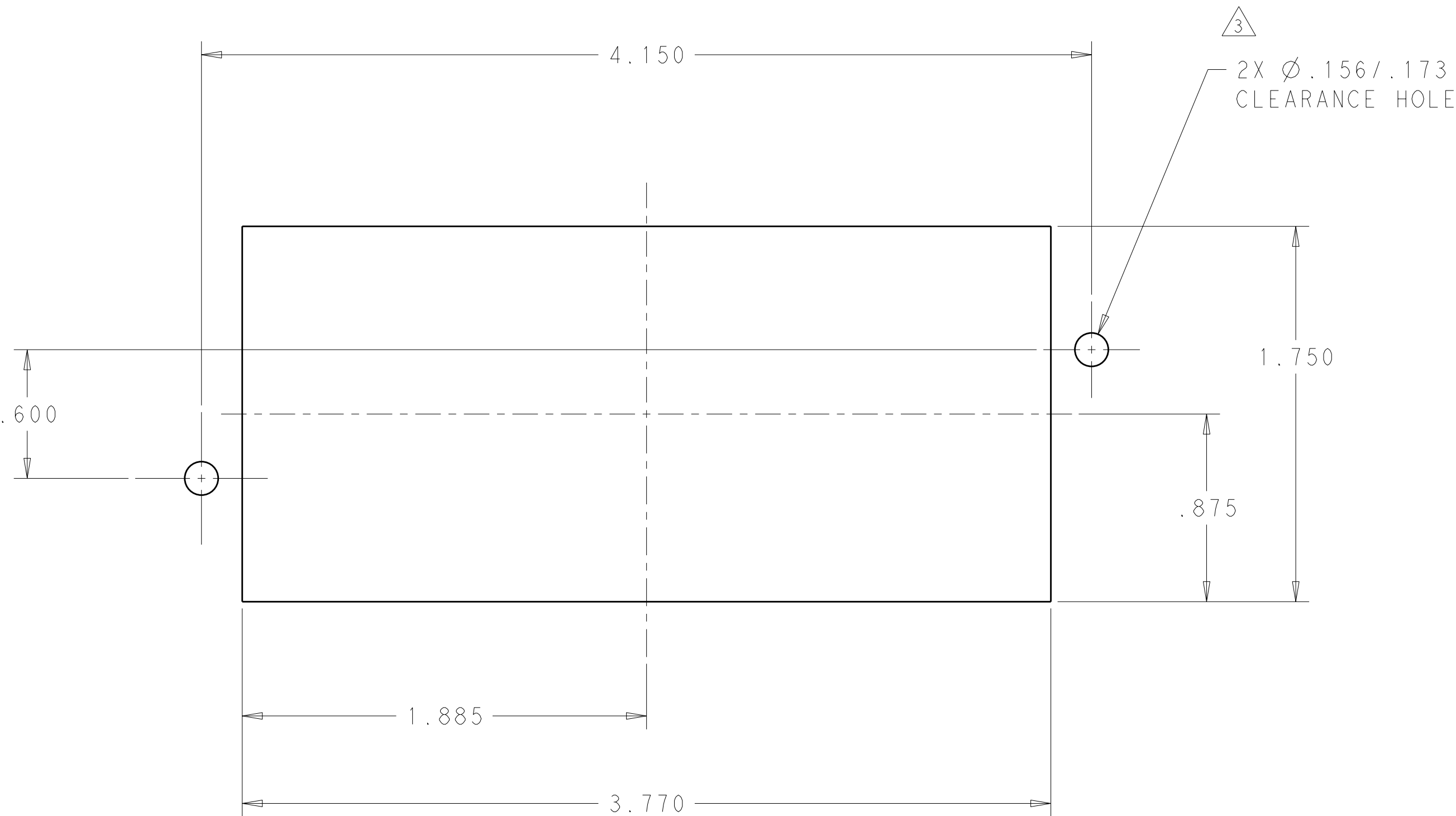
PANEL MOUNT CUT-OUT
