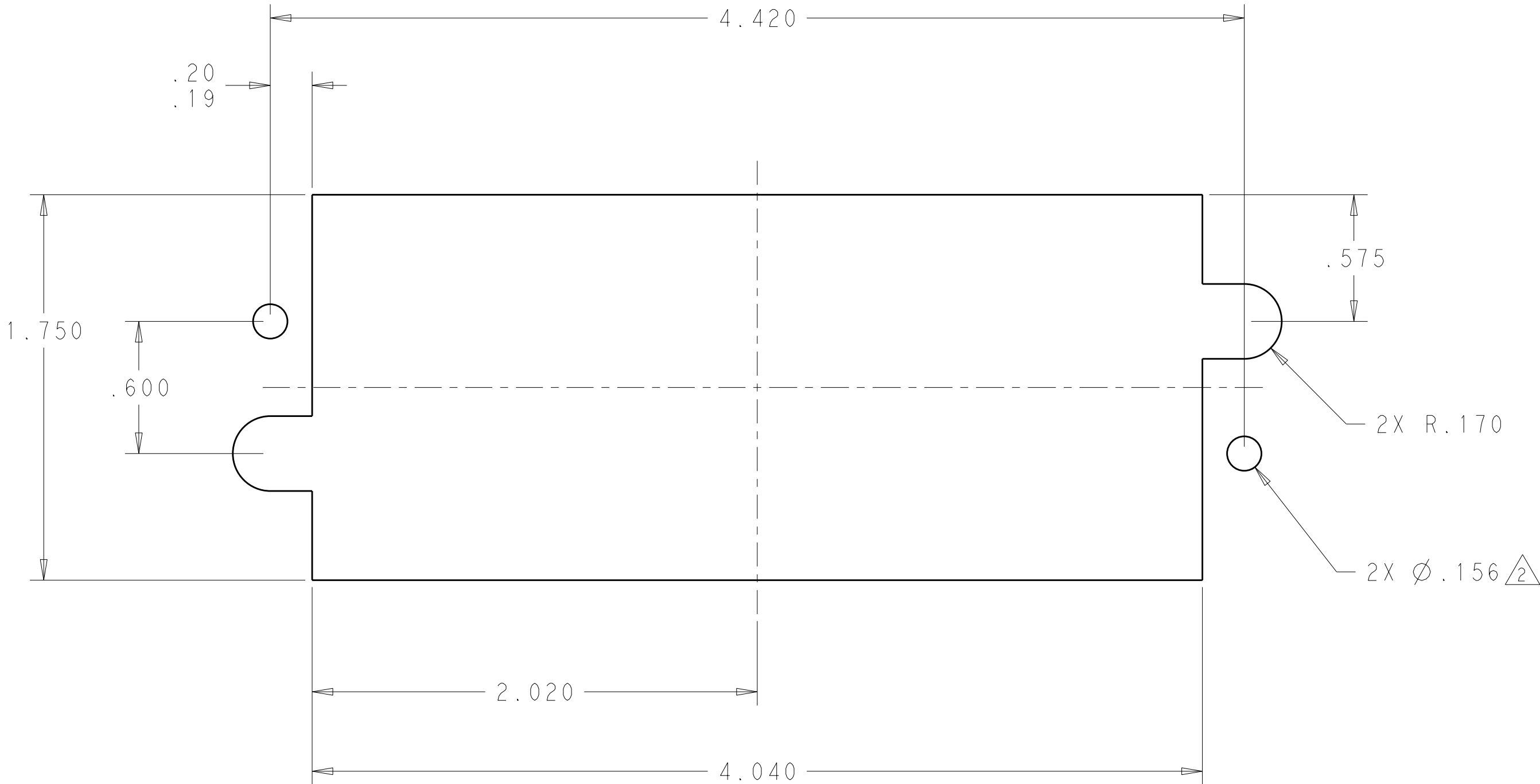
SOCKET PANEL MOUNT CUT-OUT
