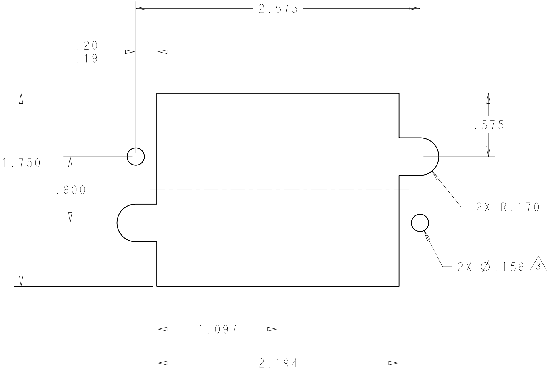
SOCKET PANEL MOUNT CUT-OUT
