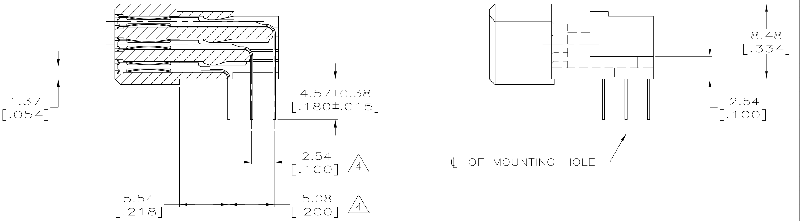
SECTION T-T
