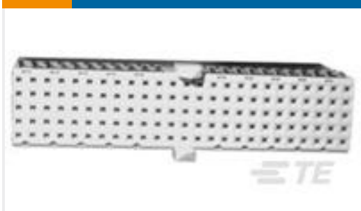
TE Part #5646574-1 Z-PACK A/B REC ASY 125P 2MMHM
