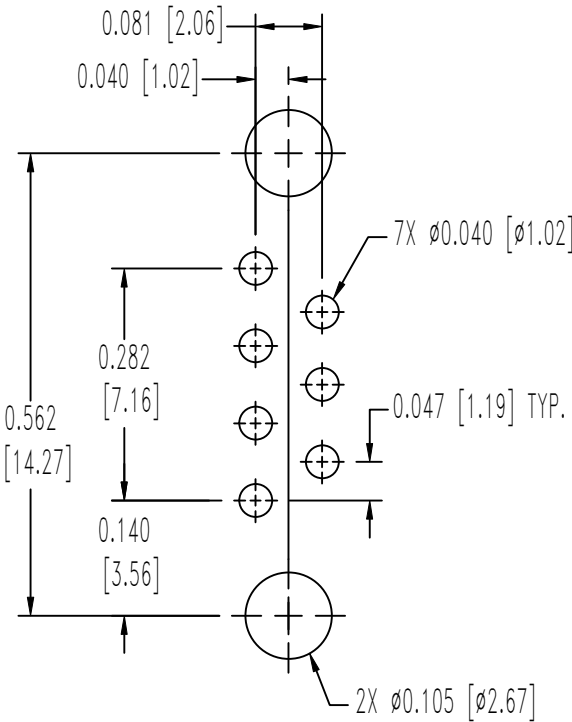
CONTACT HOLE PATTERN
