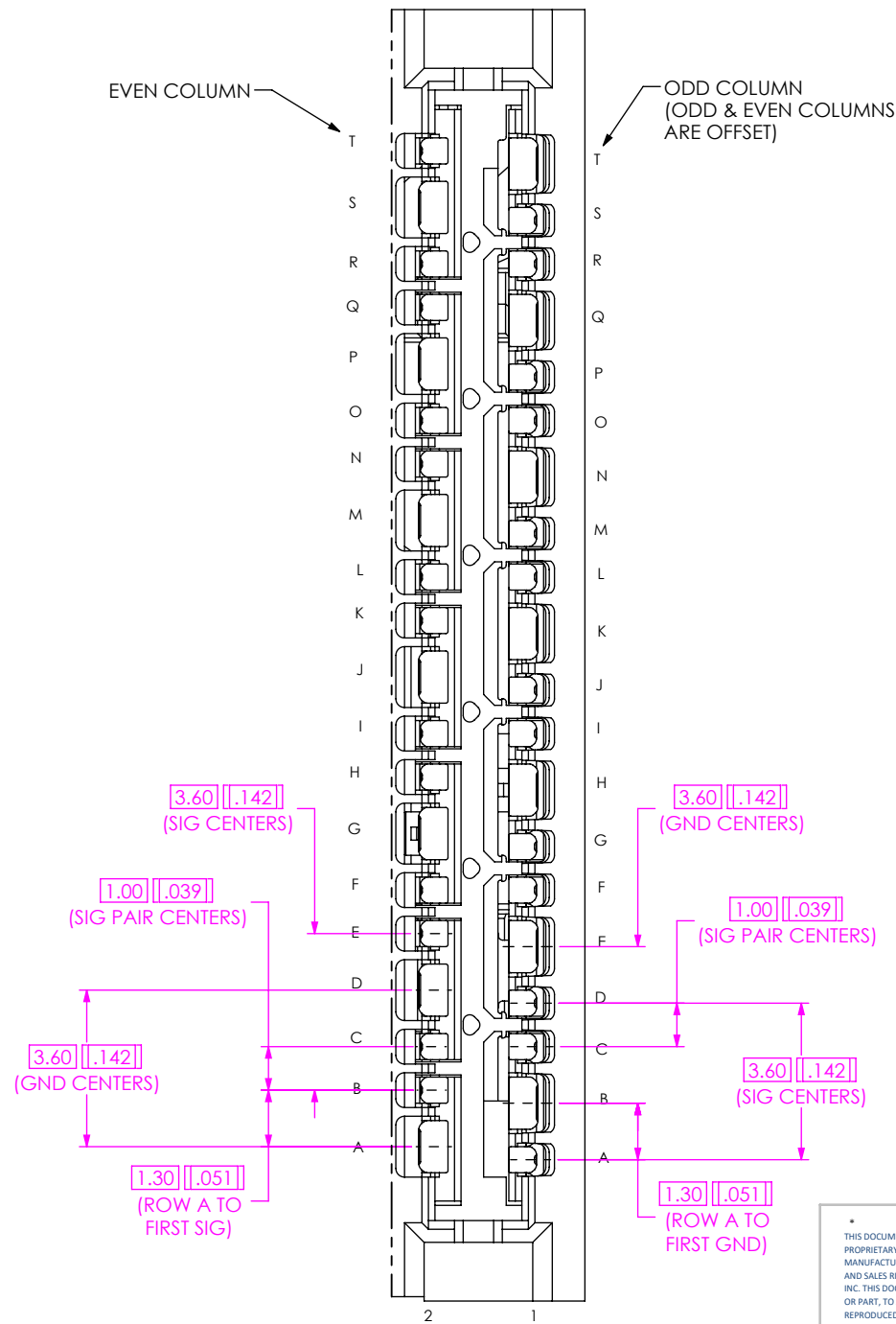
DETAIL 'A' SCALE 6 : 1
