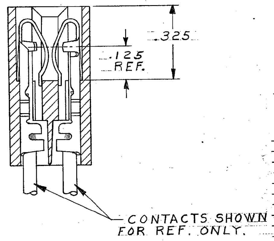
SECT. A-A
