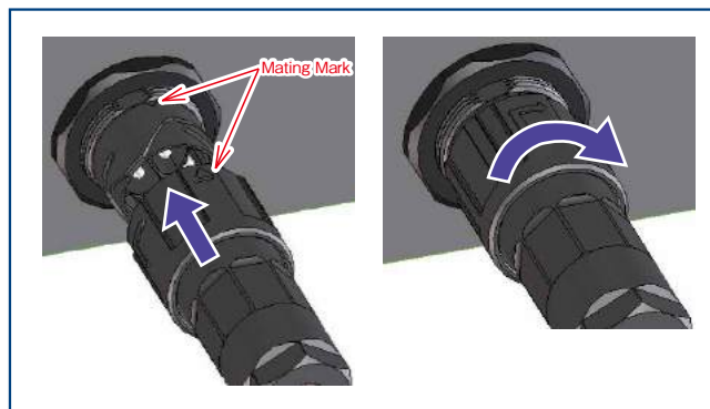
Bayonet Lock
