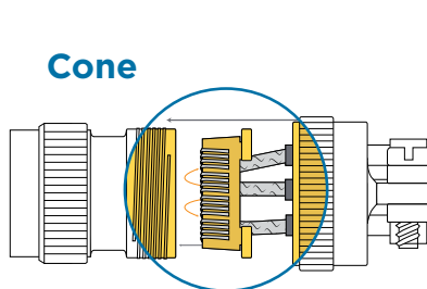
Braid/Pigtails clamped between cones Used on: 64/308/HexaShield Series
