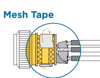
Wraps mesh tape wraps around individual screens to eliminate EMC windows Used on: KMA Series
