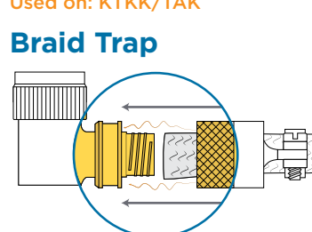
Braid trapped in loose fitting thread Used on: 95/77 Series
