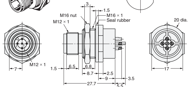
(Solder Cup Pins)
