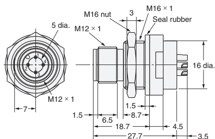
(Solder Cup Pins)
